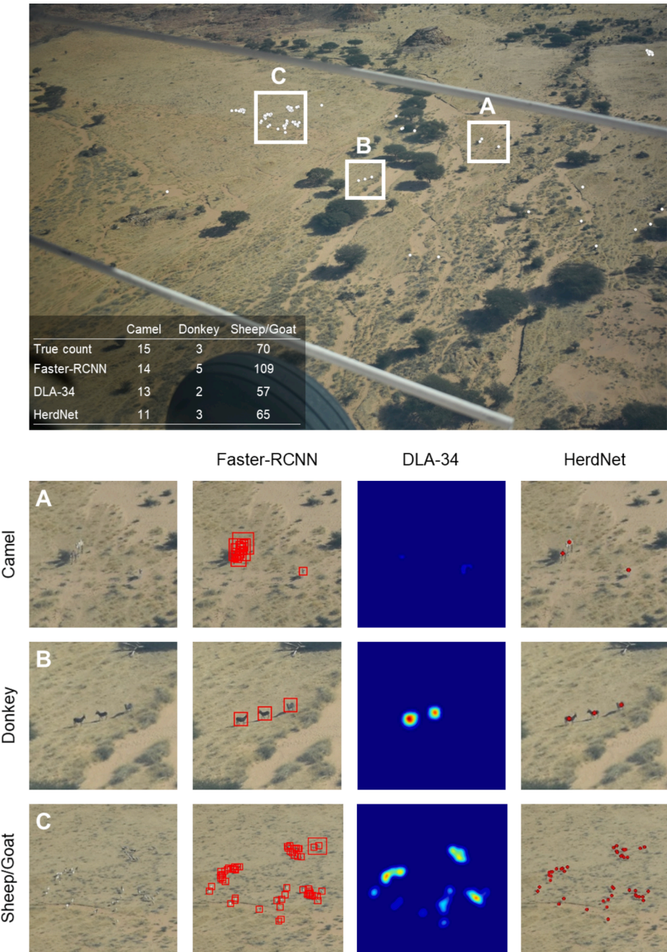
Fig. 5. Predictions of the three trained architectures on a 24-megapixel image containing the three target species (camel, donkey, and sheep/goat). White points correspond to the annotations, red bounding boxes to Faster-RCNN predictions, density maps to the predictions of adapted DLA-34, and red points indicate the HerdNet predictions. For interpretation of the references to color in this figure legend, the reader is referred to the web version of this article. (For interpretation of the references to color in this figure legend, the reader is referred to the web version of this article.)
